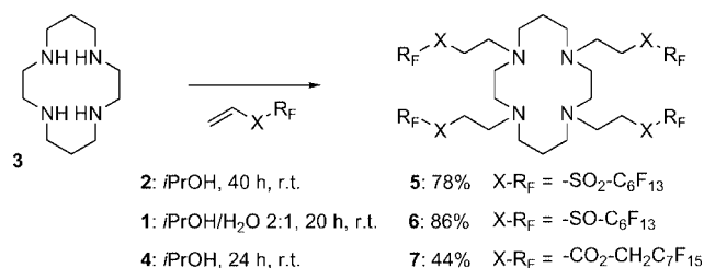
Scheme 1. Synthesis of fluoro-ponytail tetraazatetracyclotetradecanes.
