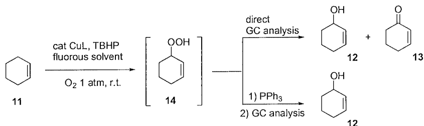
Scheme 3. Catalytic oxidation of cyclohexene.
