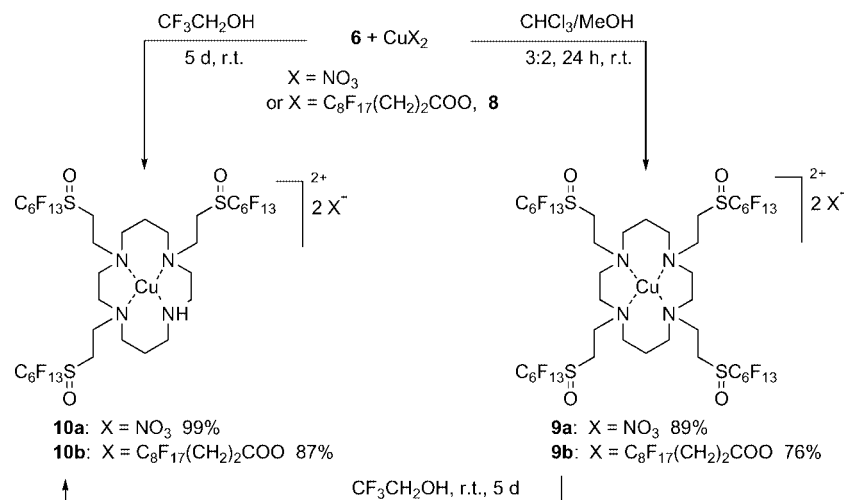
Scheme 2. Preparation of perfluorinated copper(II) complexes 9a,b and 10a,b .
